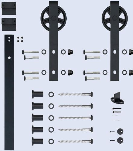
This application uses 2 Large Spoke Wheel Hook Strap Kits with 5 By-Pass Door Brackets
